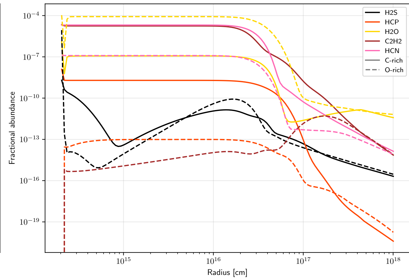
Fractional abundances - complete_model_Mdot1e-5_15kms
