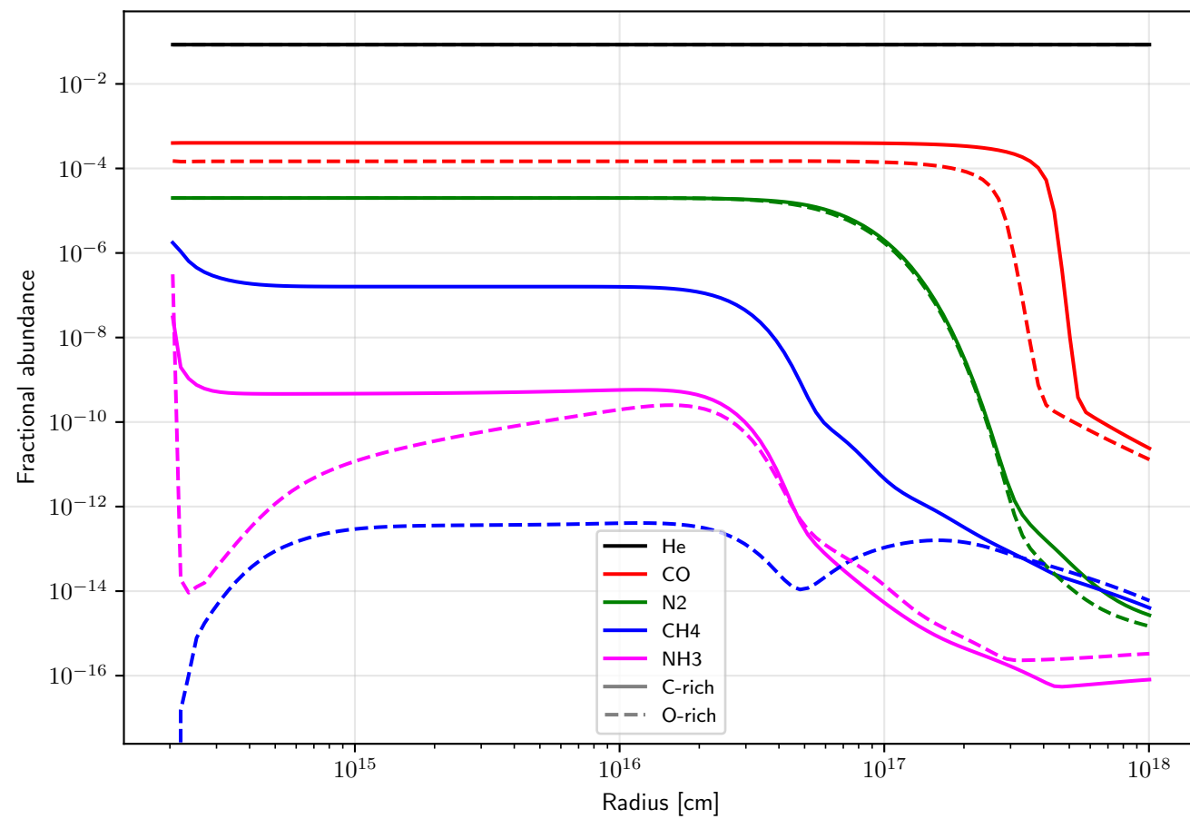
Fractional abundances - complete_model_Mdot1e-5_15kms
